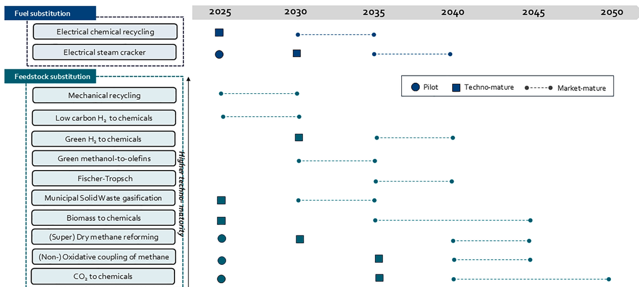
Figure 4. Projected development timeline and maturity levels of key technologies for fuel and feedstock substitution in the chemical industry, based on author's synthesis
