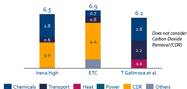
Figure 2. Estimated global supply and demand of sustainable CO 2 in 2050 across multiple scenarios
